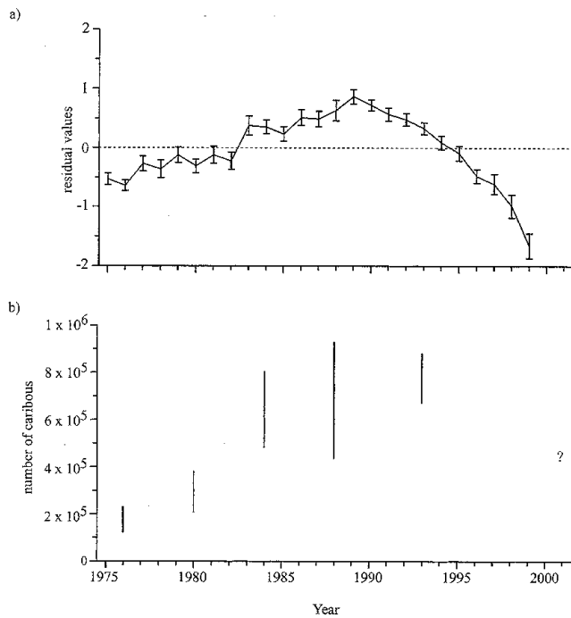
FIGURE 5. Demographic trends of the George River herd inferred with tree-ring data and the photo censuses. (a) Curve of the mean ( \pm SE) of the residual values of the regression for the 31 sites sampled in summers 1999 and 2000. (b) 90% confidence intervals of the 1976, 1980, 1984, 1988, and 1993 photo census. The question mark shows the 2001 preliminary census result. (From Couturier et al., 1990, 1996; Crête et al., 1991.)
